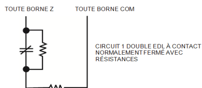
Figure 1-4 Câblage DEDL
