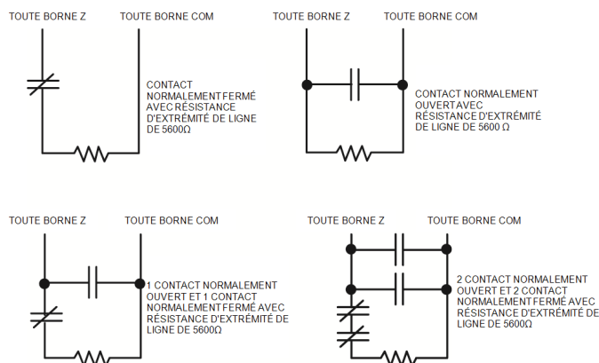
Figure 1-3 Câblage SEDL
