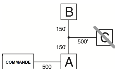
Figure 1-1 Câblage Corbus
