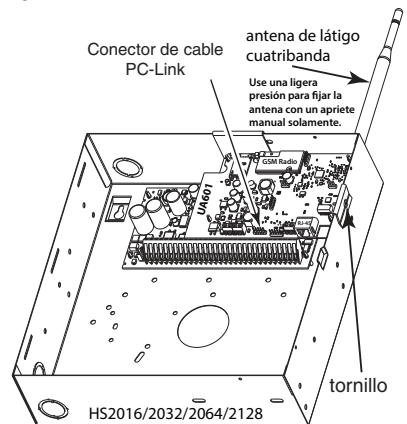
Figura 2: Panel de control HS2016/2032/2064/2128
