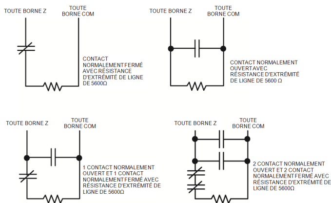
Figure 1-3 Câblage SEDL
