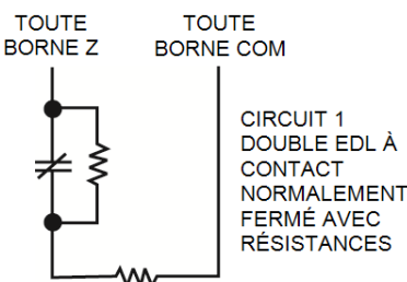
Figure 1-4 Câblage DEDL
