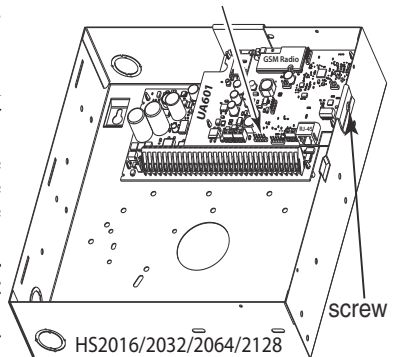
Figure 2: HS2016/2032/2064/2128 Control Panel PC-Link cable connector
