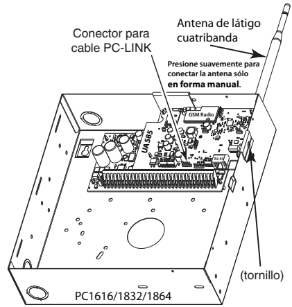
Figure 2: Panel de control PC1616/1832/1864
