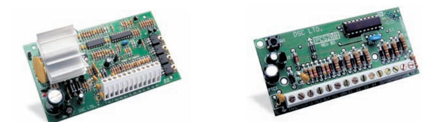
PC5200/PC5204 POWER SUPPLY MODULES PC5208 PROGRAMMABLE OUTPUT MODULE
