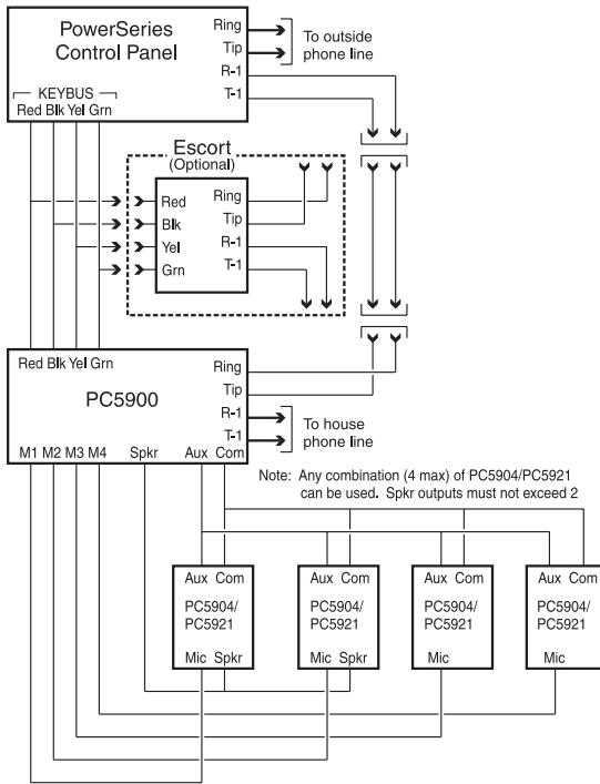
Figure 3: Wiring Details
