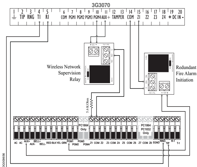
Figure 8 -Connection Details for Wireless Network Supervision Relay and Redundant Fire Alarm Trans- mission
