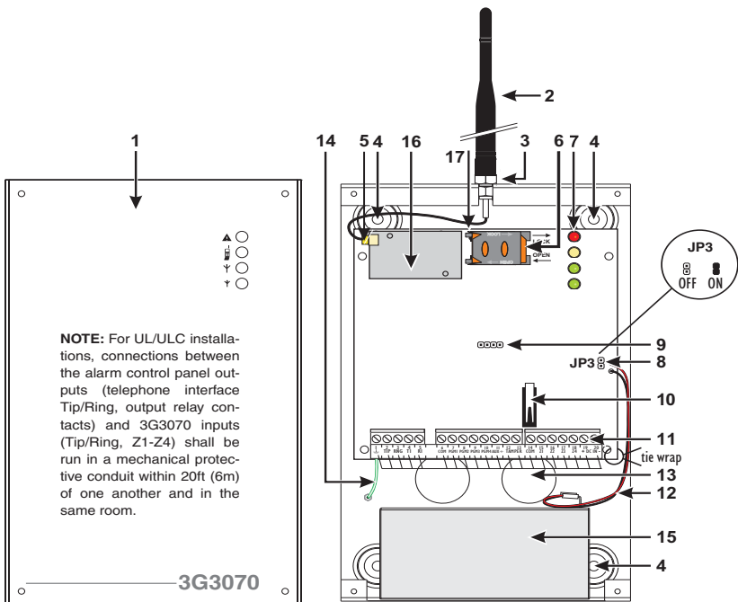
Figure 1 - Parts
