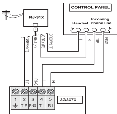
Figure 3 - Telephone Connection
