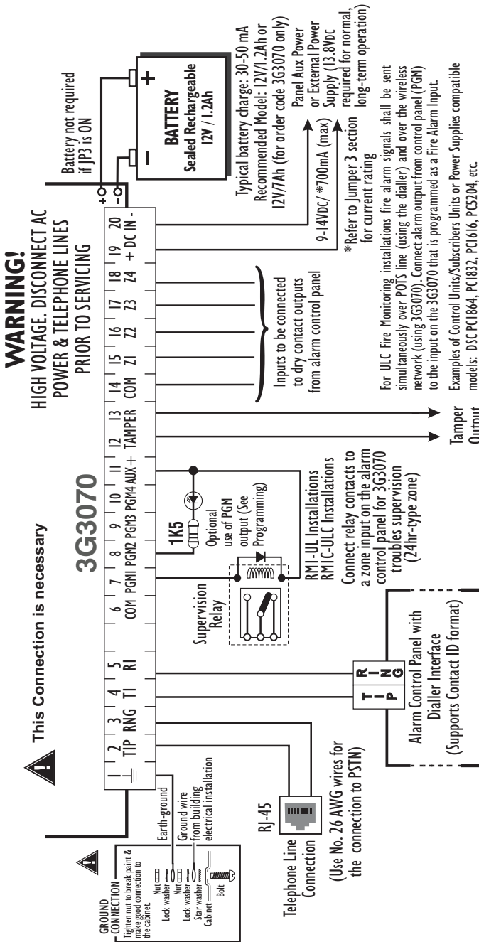
Figure 2 - Wiring Diagram
