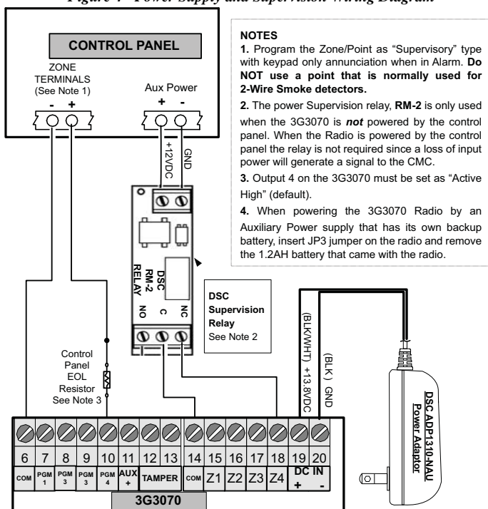
Figure 4 - Power Supply and Supervision Wiring Diagram
