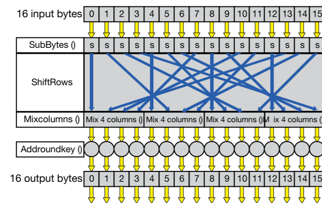
AES Transformations Round
