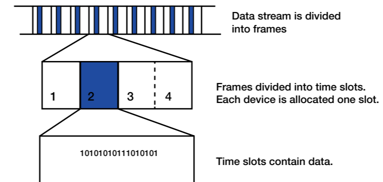
TDMA Frame Structure
