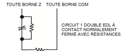
Figure 1-4 Câblage DEDL
